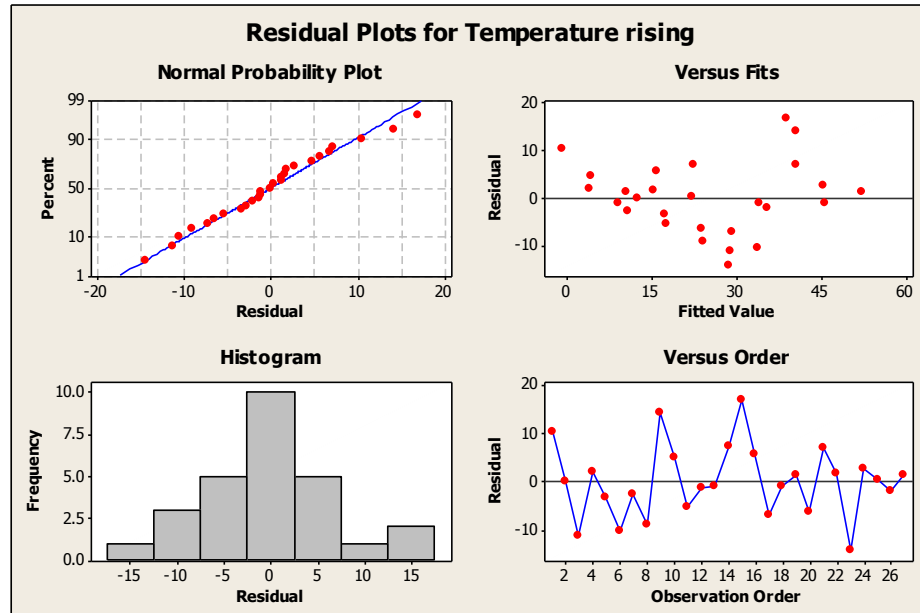
Figure 4 Residual plots temperature rising with regression model
