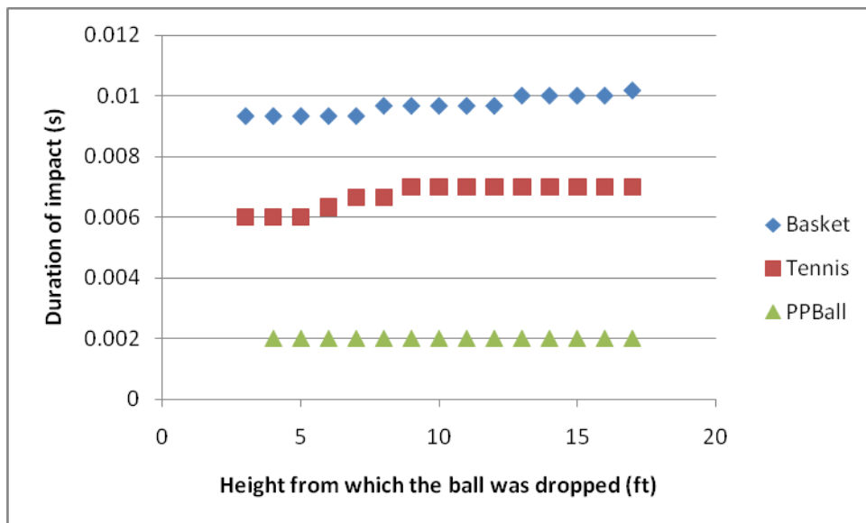
Figure 7: Duration of the impacts vs. drop heights.
