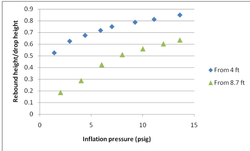
Figure 6: Height ratios vs. inflation pressures for two drop heights.
