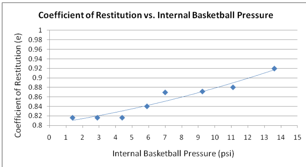
Fig. 5. The coefficient of restitution vs. internal pressure of the basketball at 4 ft.
