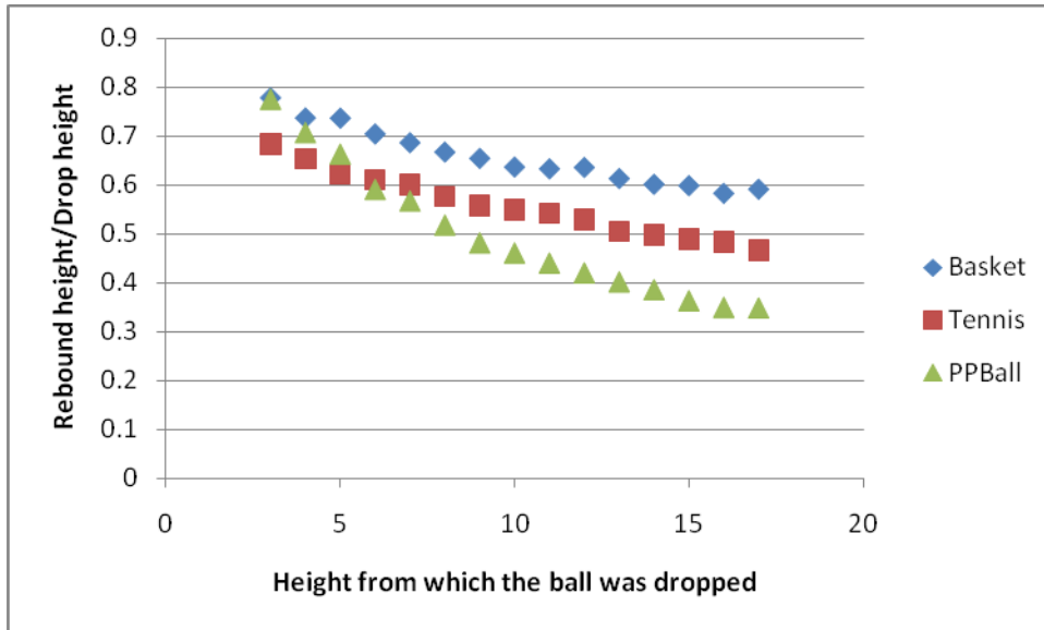
Figure 2: Variation of height ratios with drop heights (ft) (data from Group [19] ).
