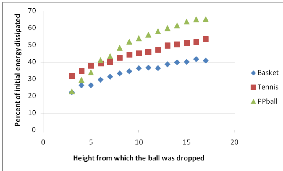
Figure 4: Percent of energy dissipated by the impacts vs. drop heights.
