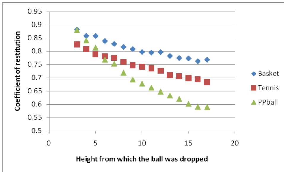
Figure 3: Variation of the coefficients of restitution with drop heights (ft).
