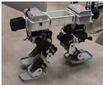
Figure 6. TWIN-GERWALK robot.
