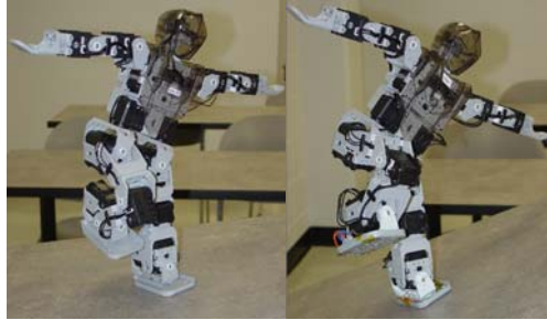
Figure 8. 1-Leg Balance using the AX-S20 (left) and the FPS (right).
