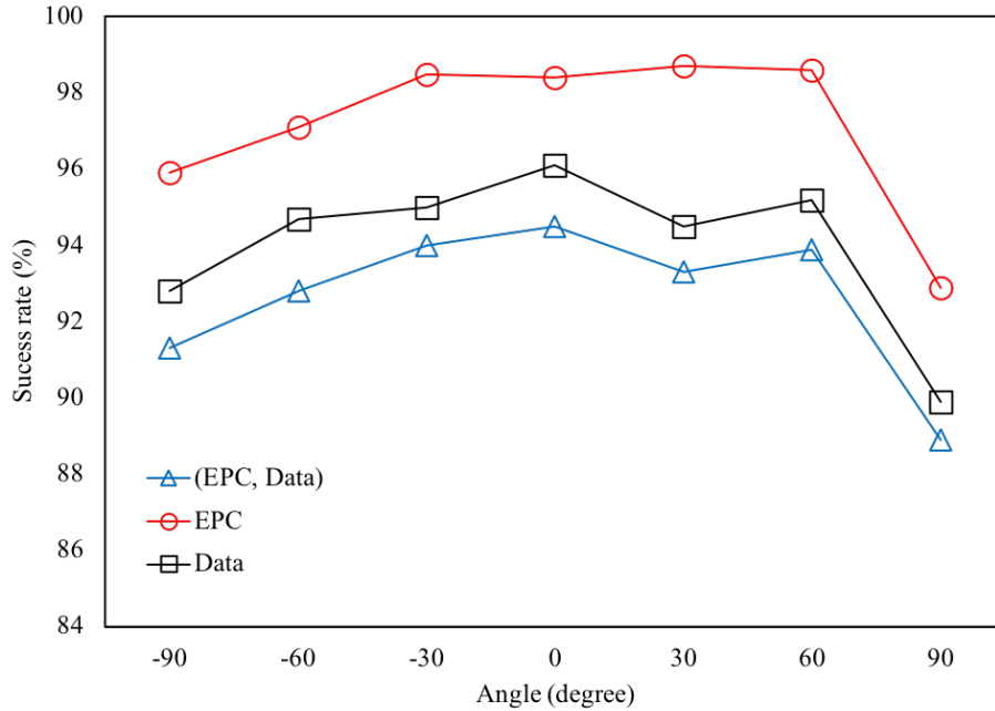
Figure 4. Successful reading rate (SR) in 7 different angle positions of tag from the reader where A_T = \{-90^\circ, -60^\circ, -30^\circ, 0^\circ, 30^\circ, 60^\circ, 90^\circ\} .
