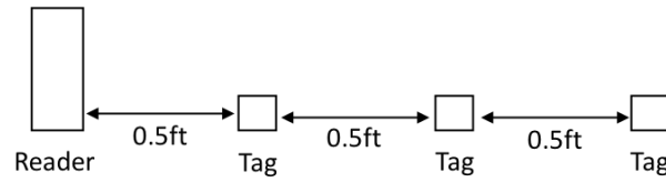
(a) Experimental setup for various position of tag in distance
