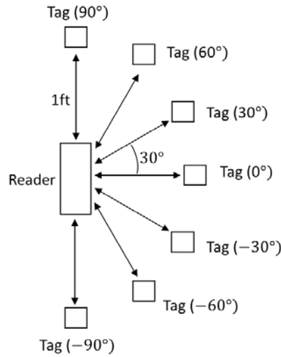
(b) Experimental setup for various position of tag in angle
