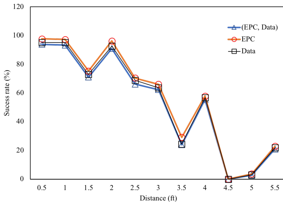
Figure 3. Successful reading rate (SR) in 11 different distance positions of tag from the reader where D = 0.5 ft to 5.5 ft.
