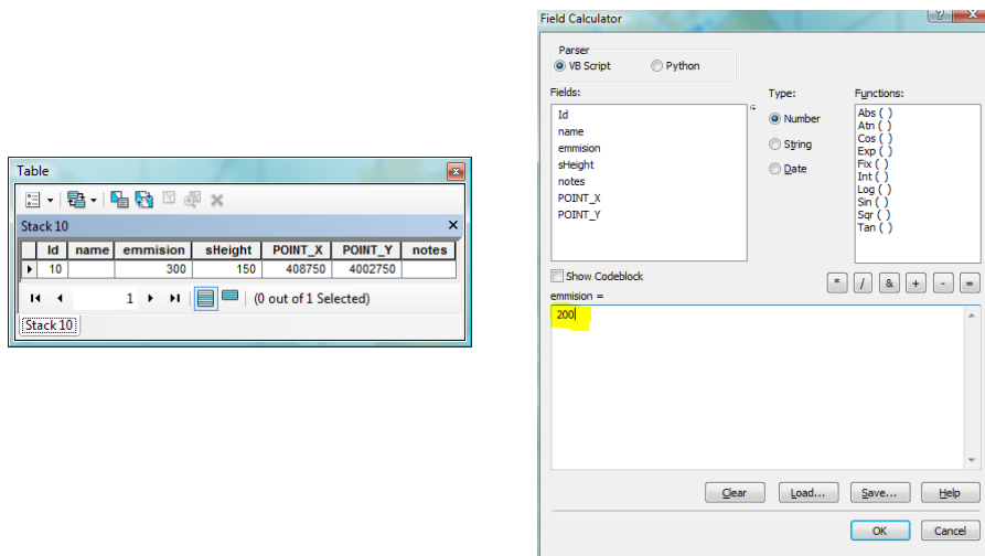
Figure 1: Interface in ArcGIS 10.0 that allows students to modify stack parameters. Students first open the attribute table for a desired stack (left picture) and right click on the heading of the stack characteristic they want to change. The table on the right then appears which allows students to update the stack height (“sHeight”) and emissions rate (“emission”).
