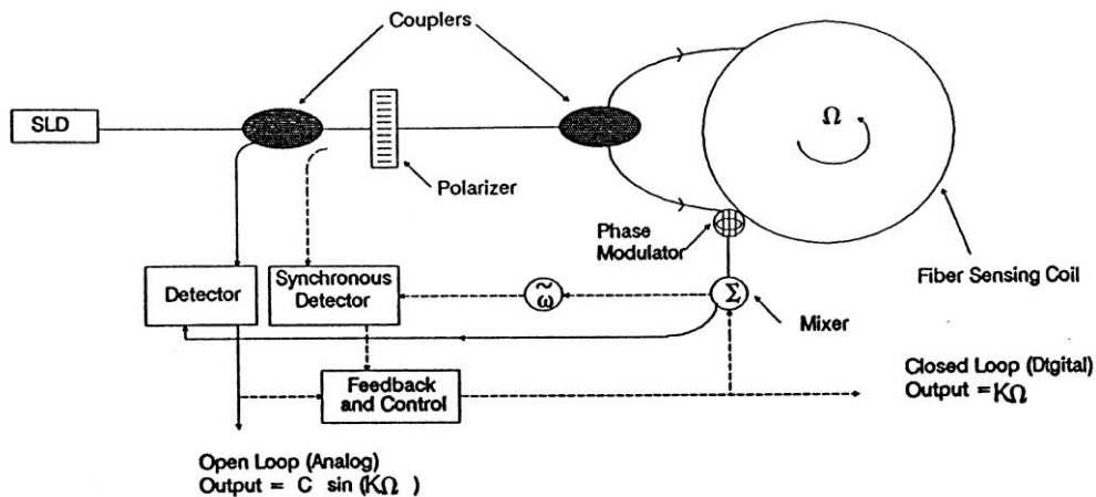
Figure 4. Interferometric fiber optic gyroscope [11]
