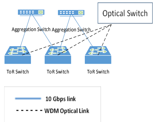
Fig. 3. Architecture of Helios data center network: Electrical/Optical Switch
