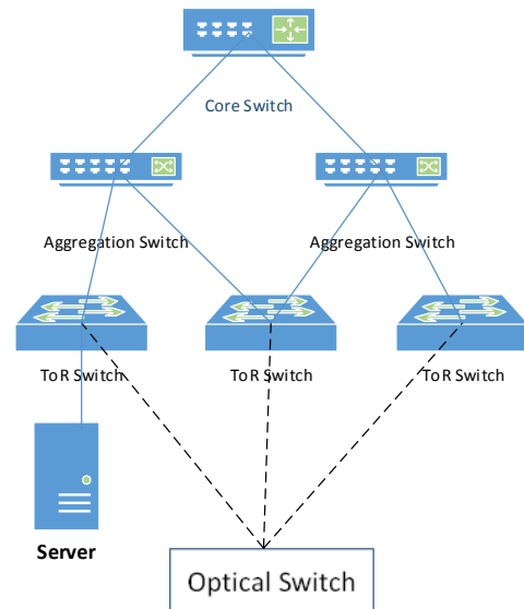
Fig. 2. Architecture of c-Through Network
