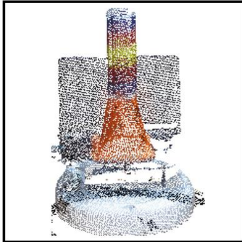
Figure 4: Updated object model using STAR technique
