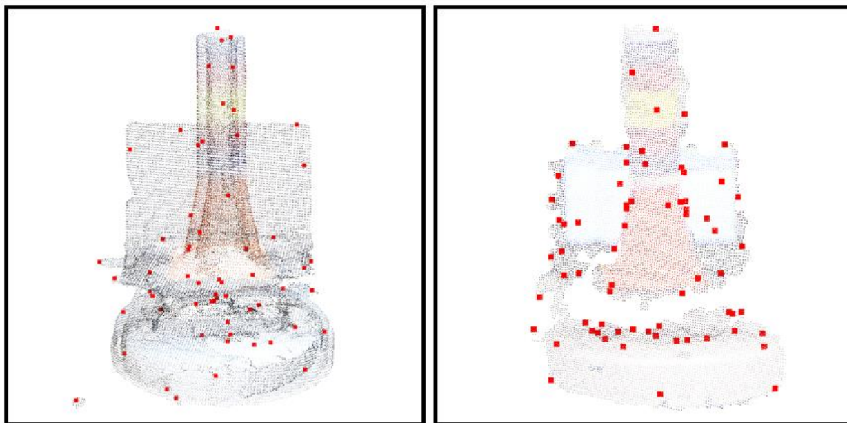
Figure 2: 3-D SIFT keypoints; Left: Create model generated by KinectFusion; Right: Create model segmented from raw data
